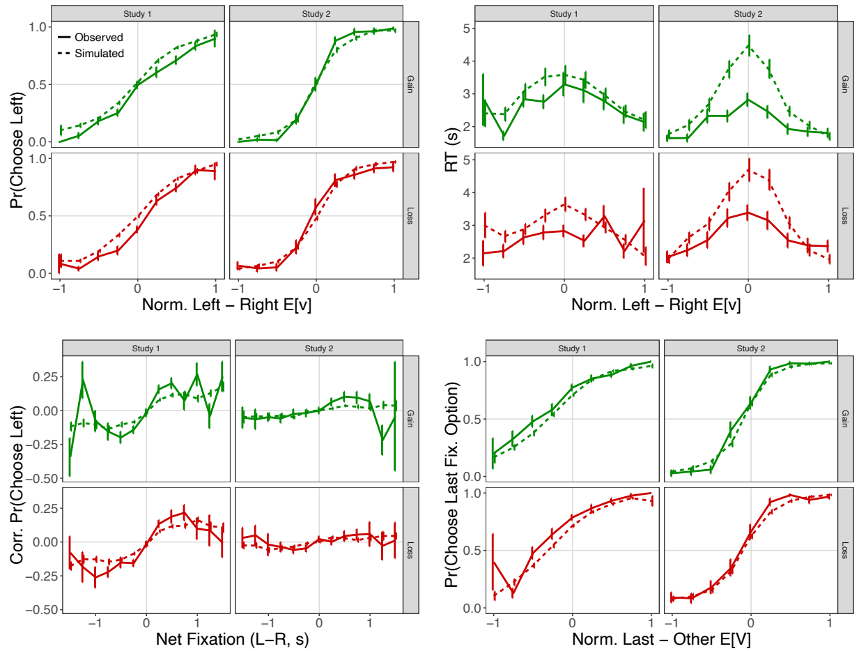
Supplementary Figure 13. AddDDM Out-of-Sample Predictions. (Top Left) The probability of choosing left as a function of the normalized relative expected value of the left option, as in Row 1 of Fig. 3. (Top Right) Response time as a function of the normalized best minus worst expected value, as in Row 2 of Fig. 3. (Bottom Left) Corrected probability of choosing the left option as a function of the net fixation time to the left option, as in Row 1 of Fig. 5. The corrected probability is computed by subtracting from each choice observation (coded as 1 if left chosen, and 0 otherwise) the proportion with which left is chosen at each relative expected value. (Bottom Right) The probability of choosing the last fixated option as a function of the normalized net expected value of the left option, as in Row 2 of Fig. 5. Rows separate the data by condition, and columns separate by study. Out-of-sample data consists of all trials divisible by 10 from all participants in joint dataset. 10 simulated datasets per participant. Error bars represent the standard error of the mean across all simulations for all participants.
